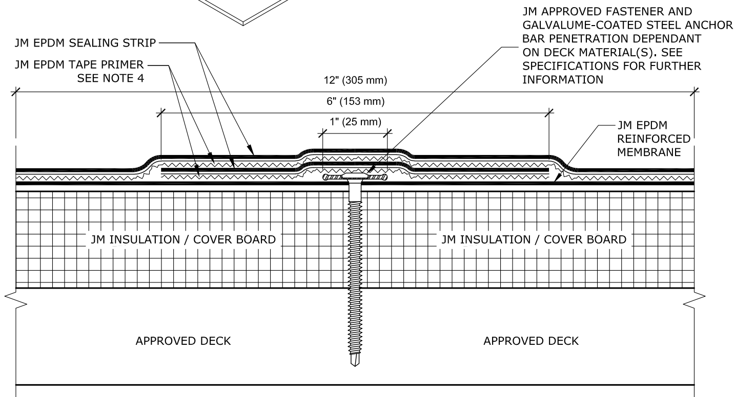
ISOMETRIC VIEW
