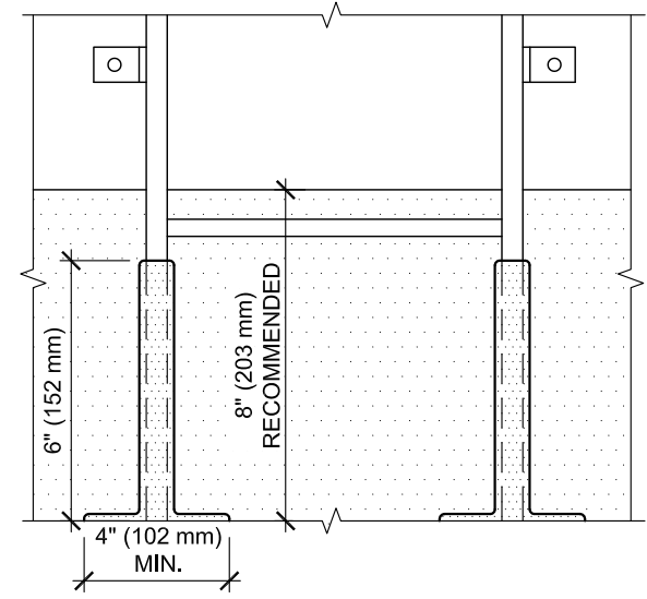
LADDER ELEVATION
