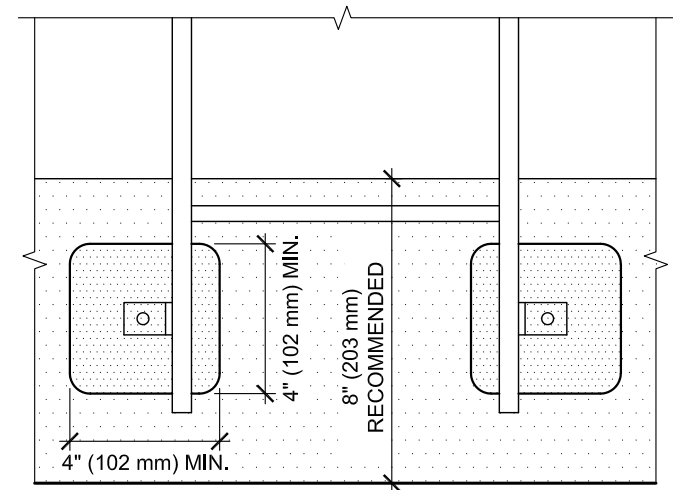
LADDER ELEVATION
