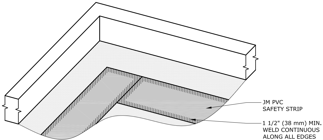
ROOF WITH PARAPET
