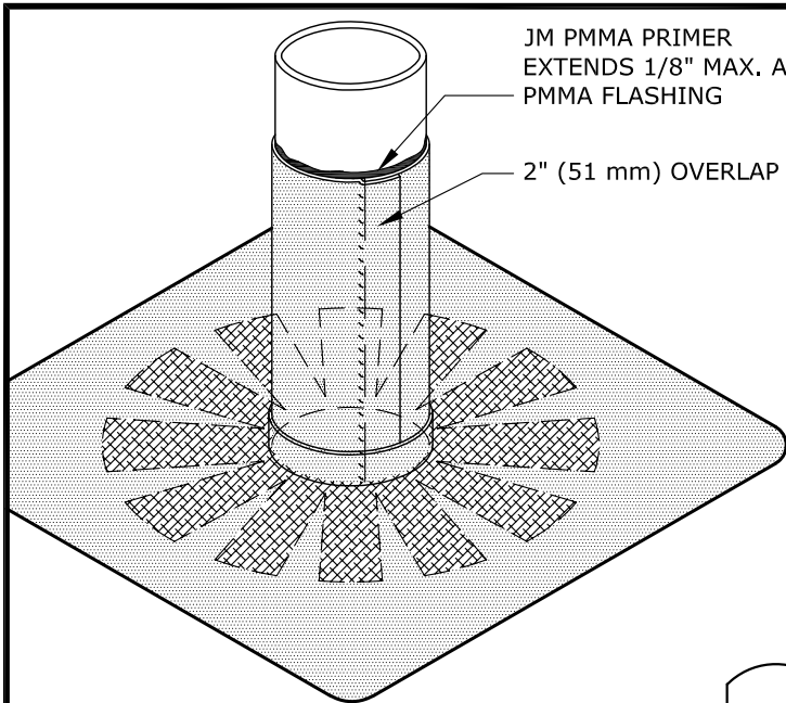
ISOMETRIC VIEW
