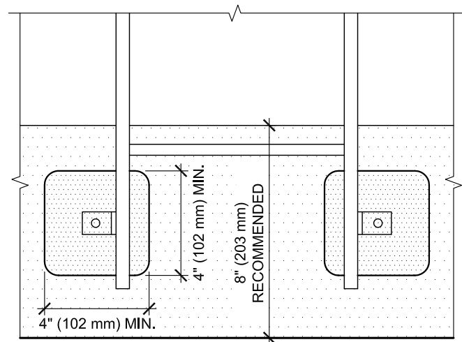
LADDER ELEVATION
