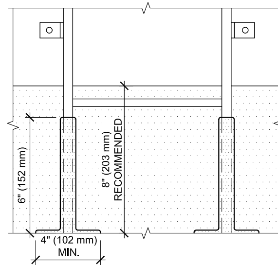
LADDER ELEVATION
