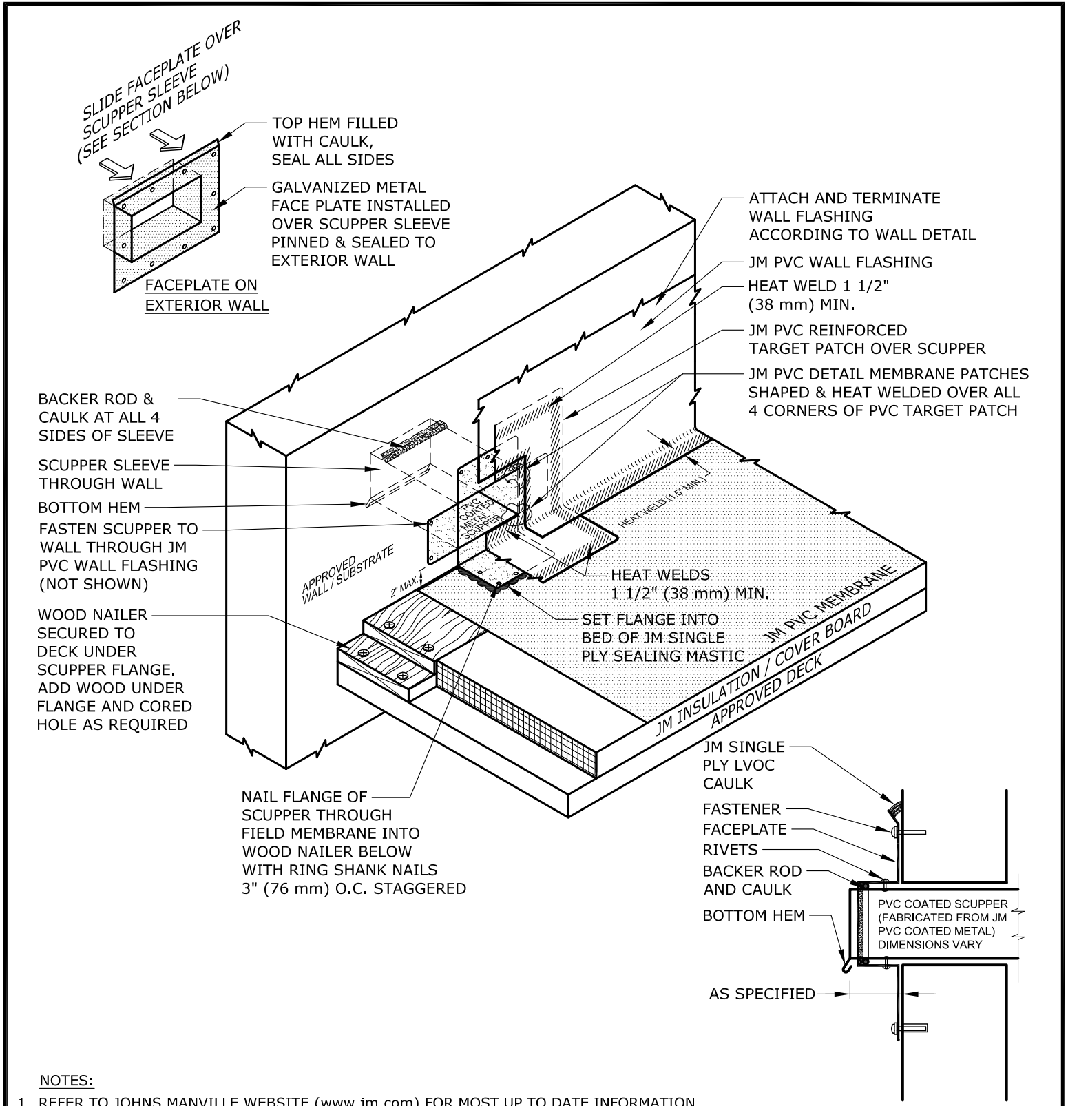
SCUPPER SECTION AT EXTERIOR WALL
